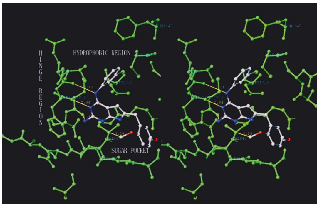
Figure 4. Stereoview: model of compound 5 superimposed on the ATP structure (not shown) in VEGFR-2.
