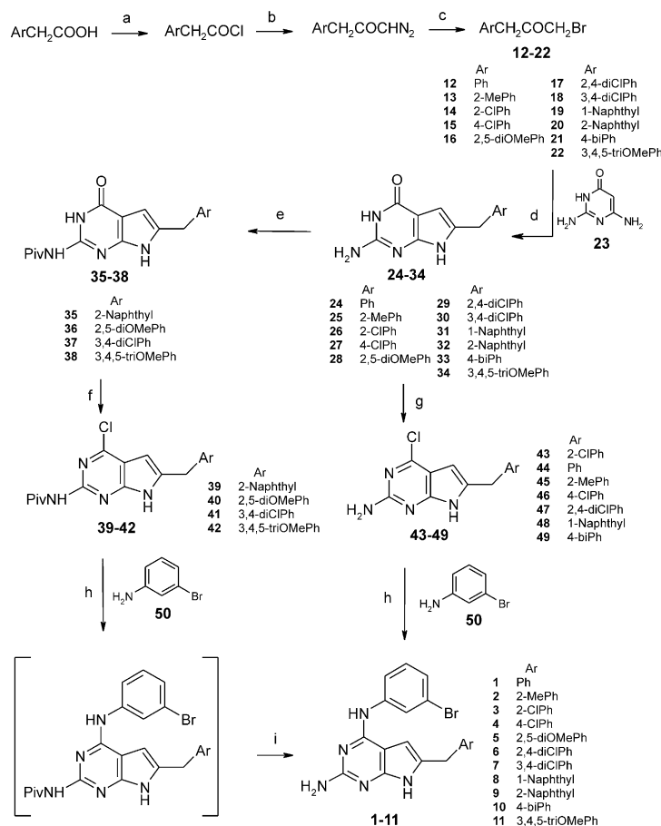
Scheme 2. (a) \text{SOCl}_2 , benzene, reflux, 1 h; (b) \text{CH}_2\text{N}_2/\text{Et}_2\text{O} , 30 min; (c) 47.5% HBr, 70–80 °C, 1 h; (d) DMF, rt, 3 days; (e) \text{Piv}_2\text{O} , DMF, DMAP, \text{Et}_3\text{N} , 60–70 °C, 2 days; (f) \text{POCl}_3 ; (g) \text{POCl}_3 , \text{PhNMe}_2 (h) i -PrOH, 2–3 drops of concd HCl, reflux, 30 min, (i) 15% KOH, 1,4-dioxane, reflux, 10 h.
