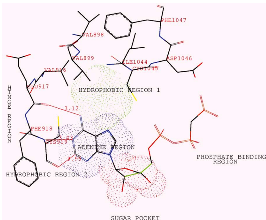
Figure 2. ATP from IRK modeled into VEGFR-2 using SYBYL 6.7.
